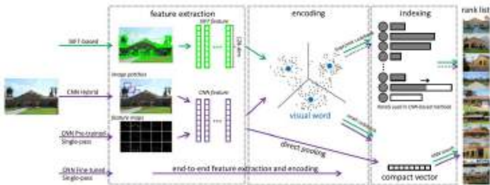
Figure 7.28 Typical pipeline for feature-based instance retrieval (Zheng, Yang, and Tian 2018) © 2018 IEEE, showing the feature extraction, encoding, and indexing portions, which are often collapsed when using a deep learning framework.
